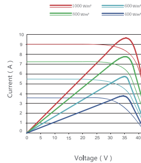
Current-Voltage & Power-Voltage Curves (305W)
